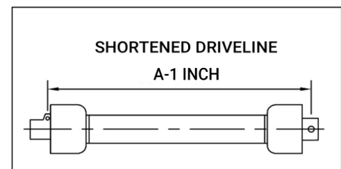
Fig. 3 SHORTENING
