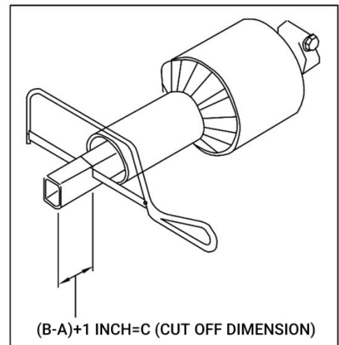
Fig. 2 CUT OFF DIMENSION
