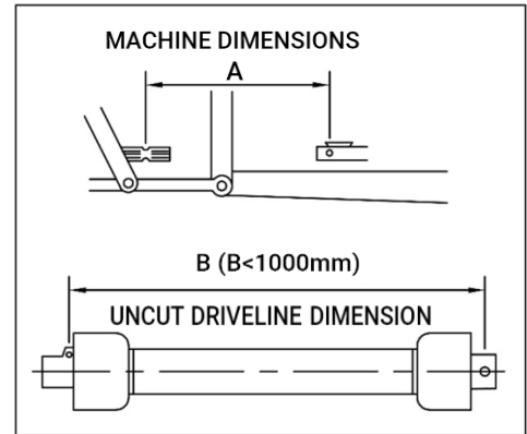
Fig. 1 DRIVELINE DIMENSION
