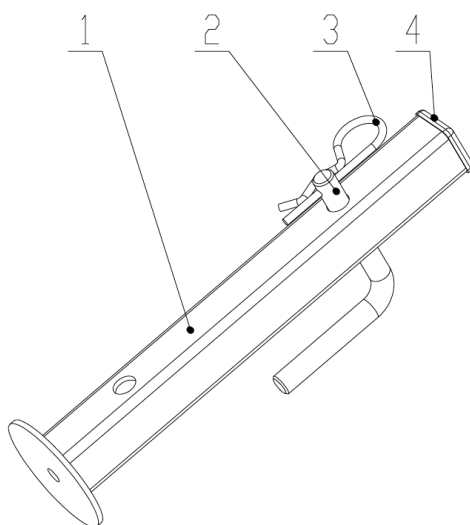
Figure 1-2: Raker Sub-Assembly
