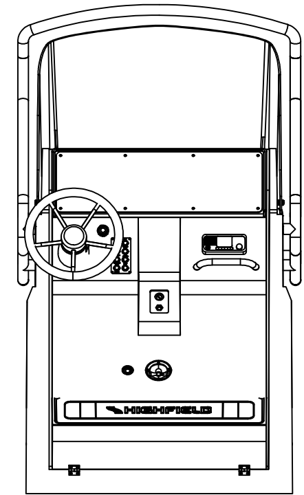
View B
