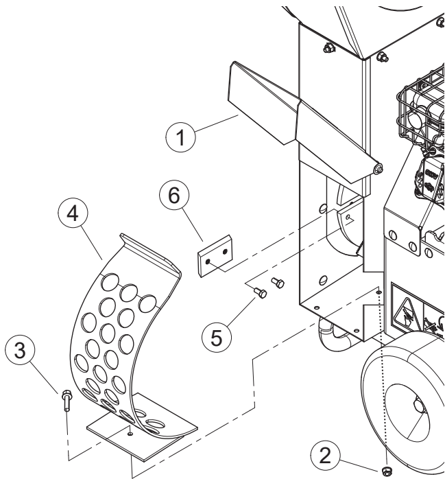
Figure 5.2, Blade Removal and Installation *SC-2013 Model Shown
