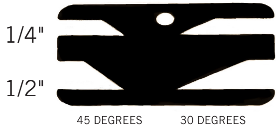
45 DEGREES 30 DEGREES Figure 5.4, Blade Angle Gauge Plate
