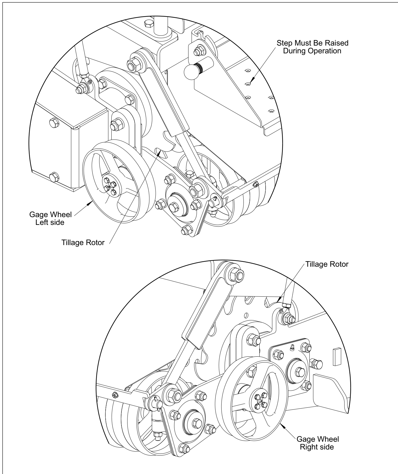
Figure 2-14: Gage Wheels
