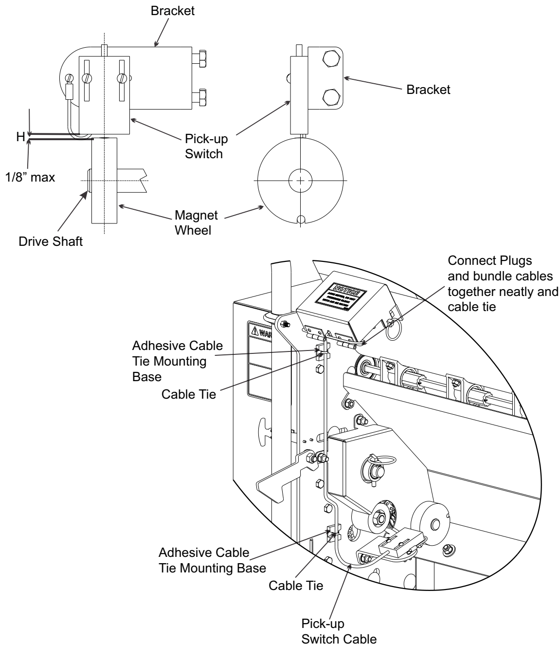
Figure 3-2: Acre Meter (2 of 2)
