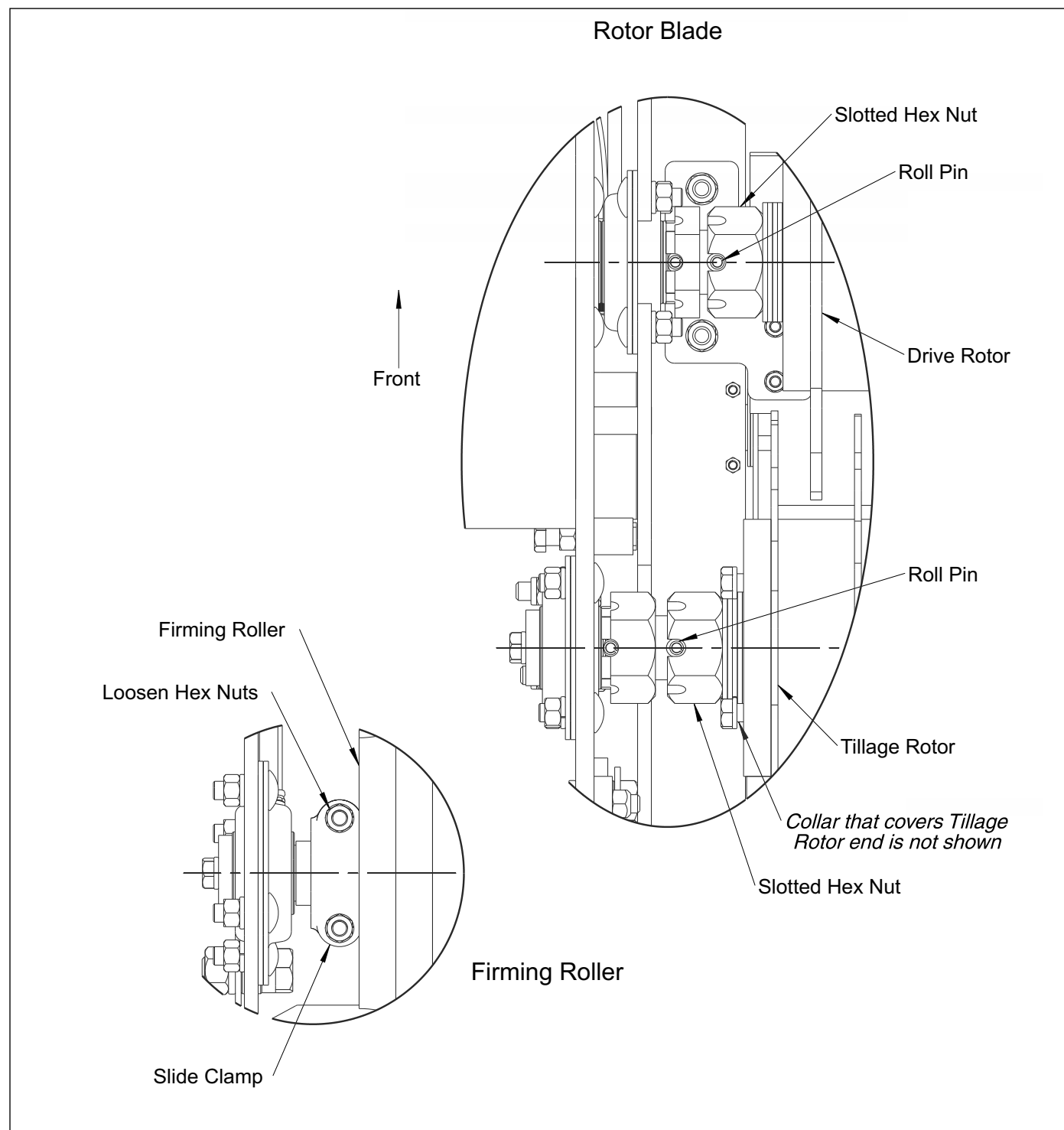
Figure 4-6: Rotor Blade and Firming Roller
