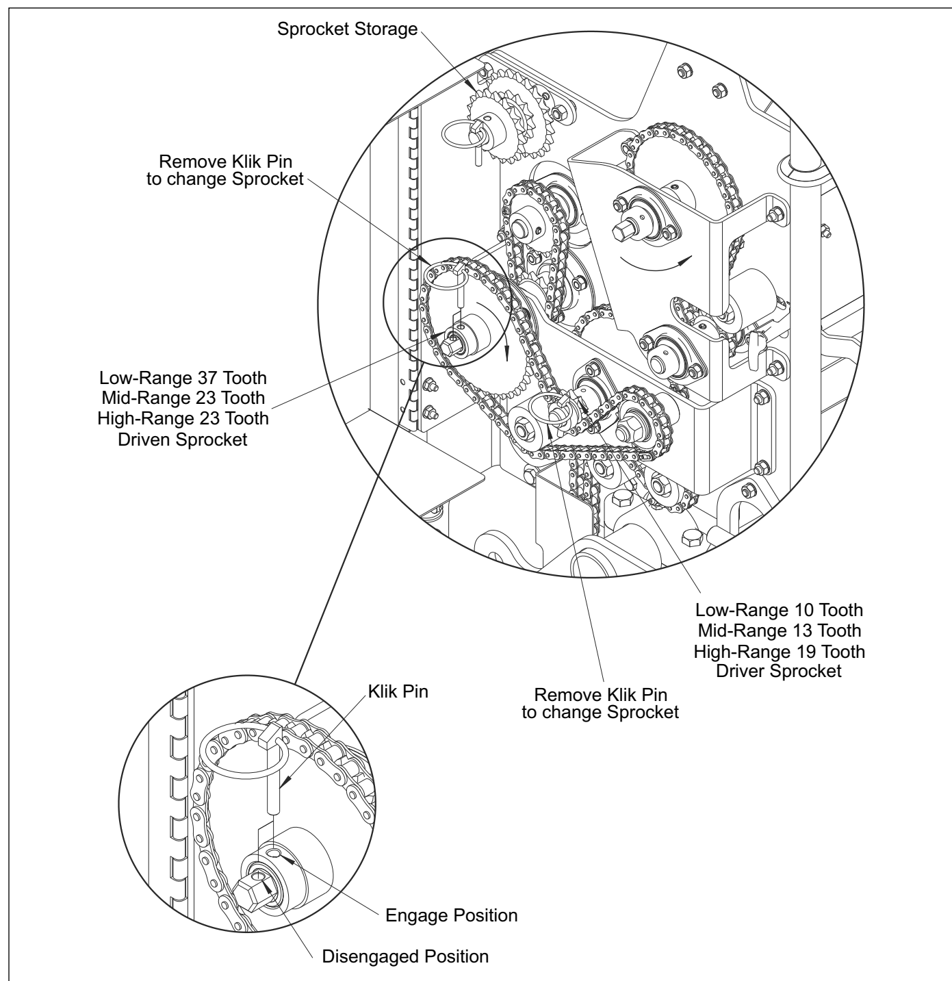
Figure 2-7: Seed Rate
