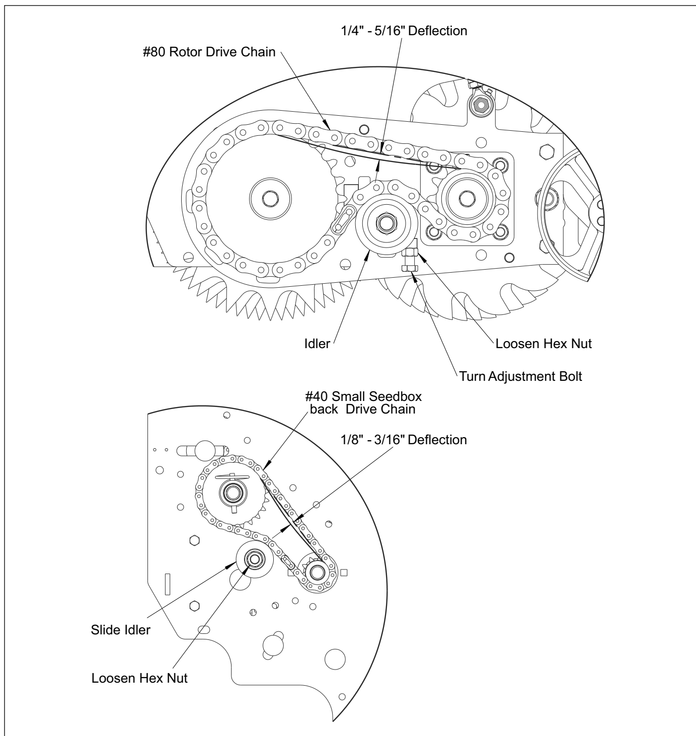
Figure 4-3: Chain Tension (1 of 2)
