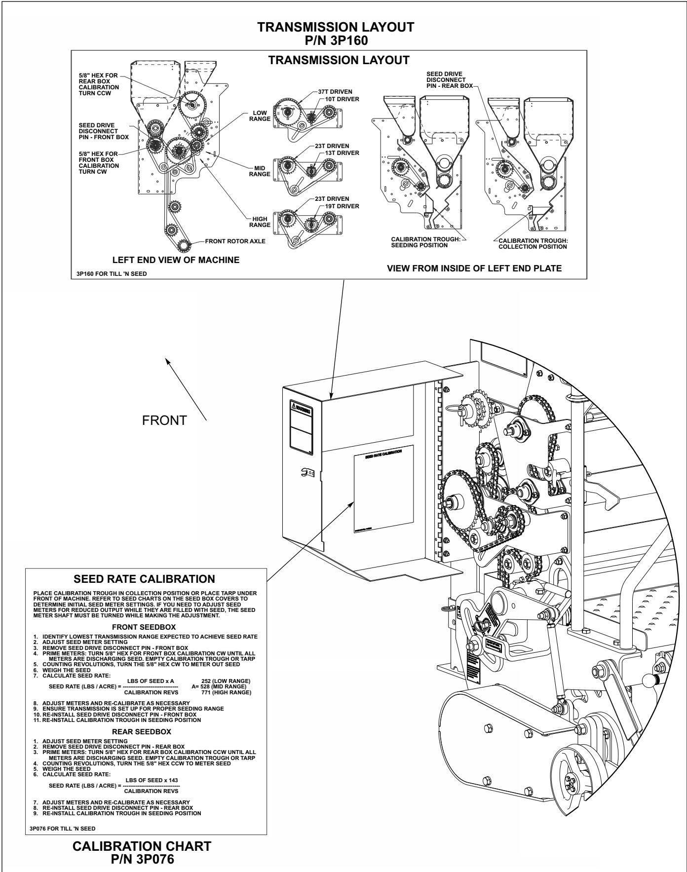
Figure 1-7: Decals (5 of 5)
