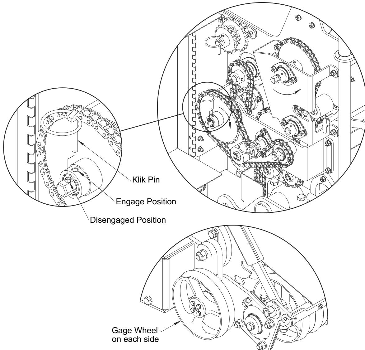
Figure 2-12: Seeding
