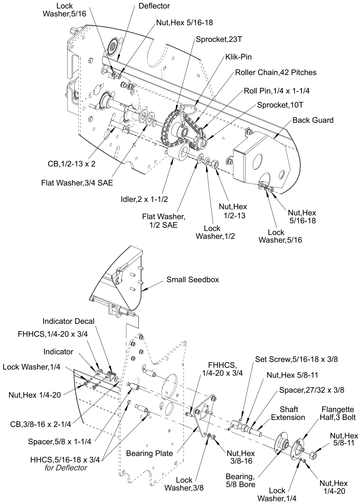
Figure 3-5: Small Seedbox Kit (3 of 3)
