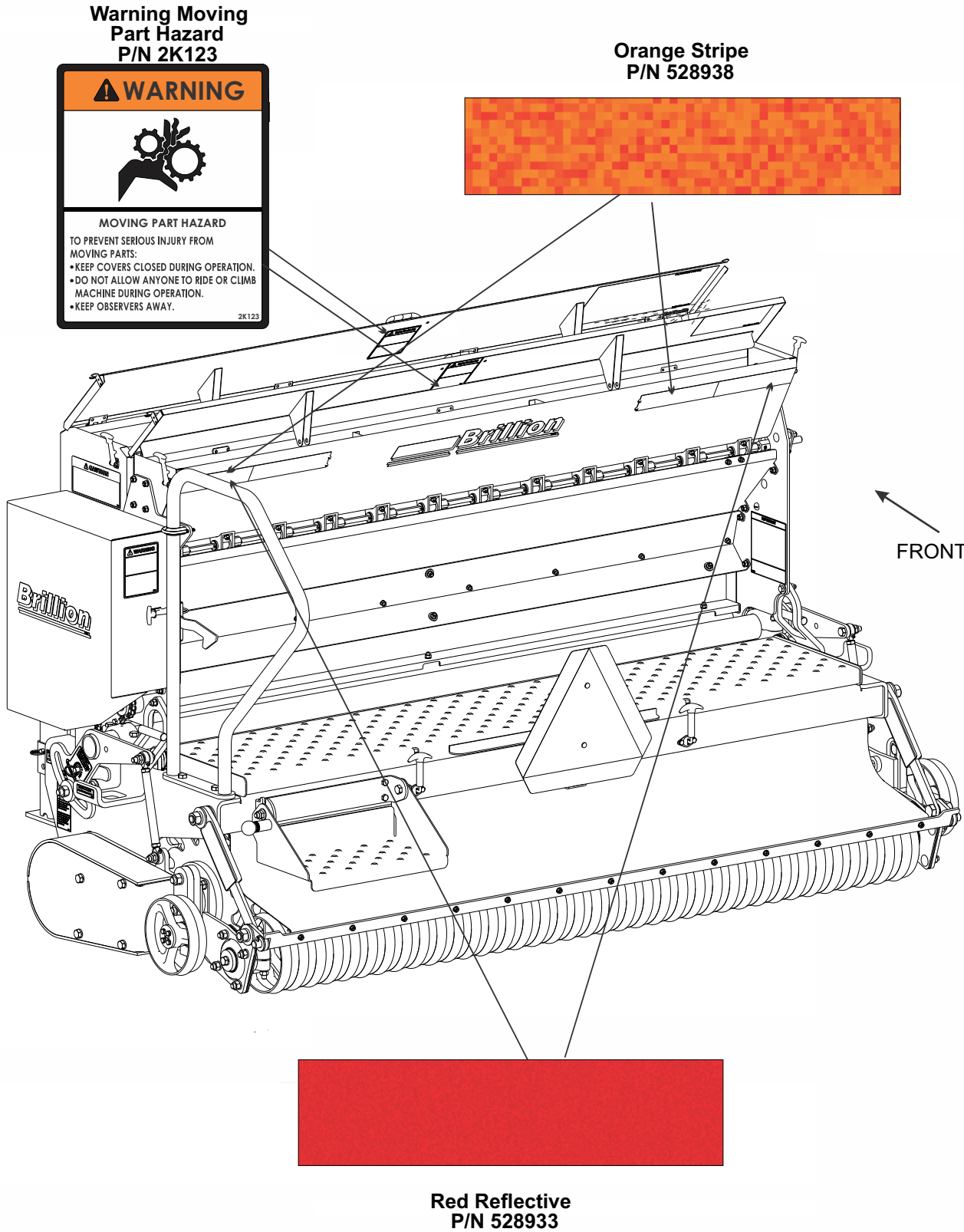
Figure 1-5: Decals (3 of 5)
