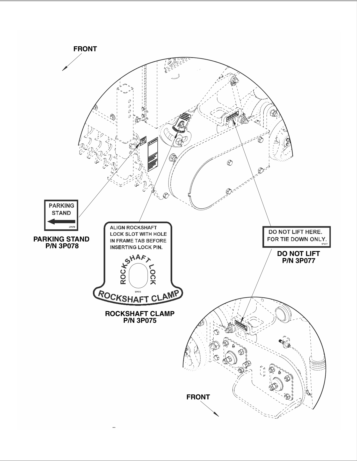
Figure 1-4: Decals (2 of 5)
