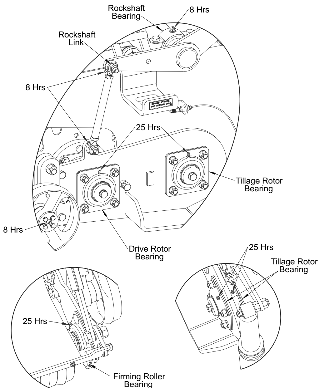
Figure 4-1: Lubrication (1 of 2)
