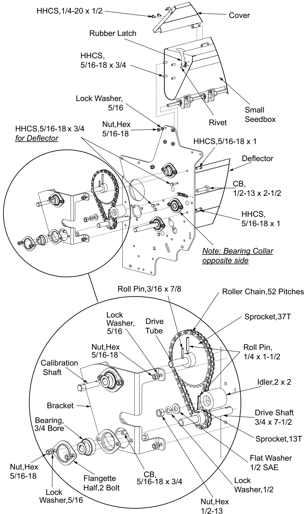
Figure 3-4: Small Seedbox Kit (2 of 3)
