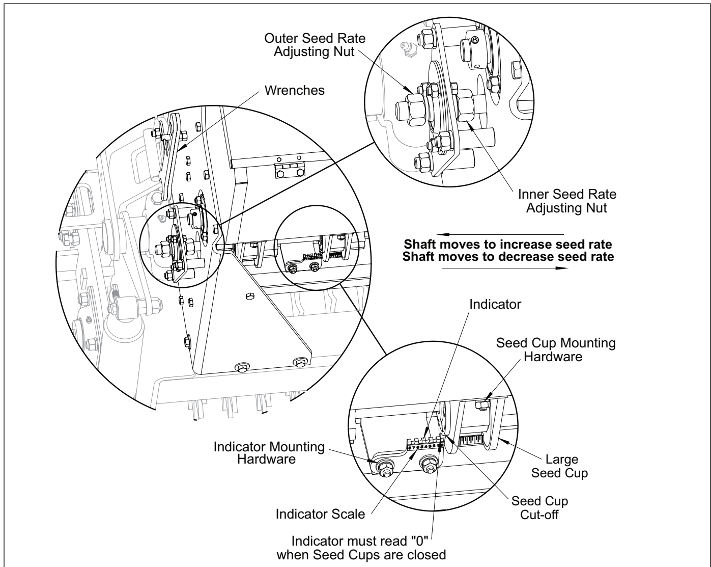
Figure 2-8: Front Seedbox Cups
