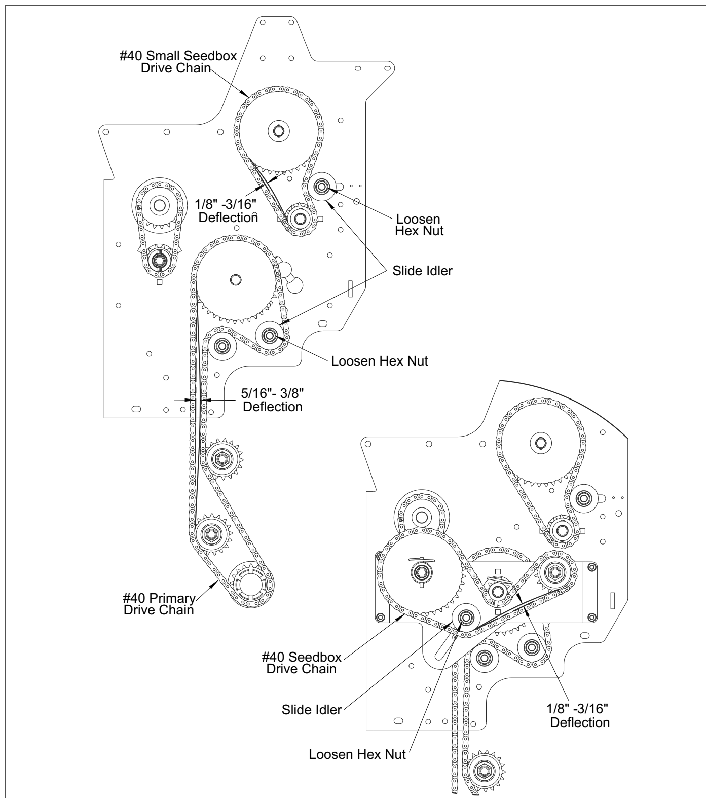
Figure 4-4: Chain Tension (2 of 2)
