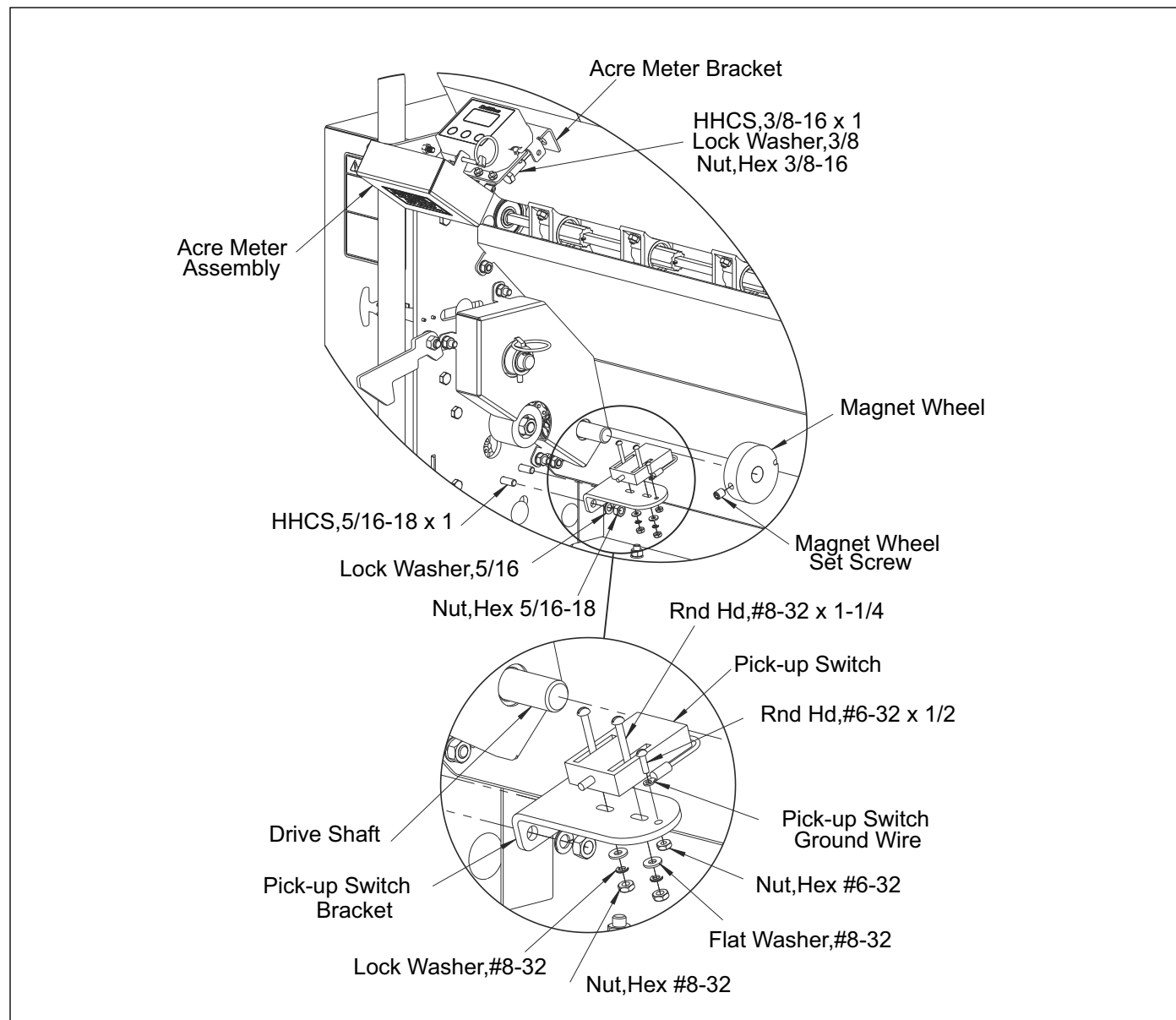
Figure 3-1: Acre Meter (1 of 2)
