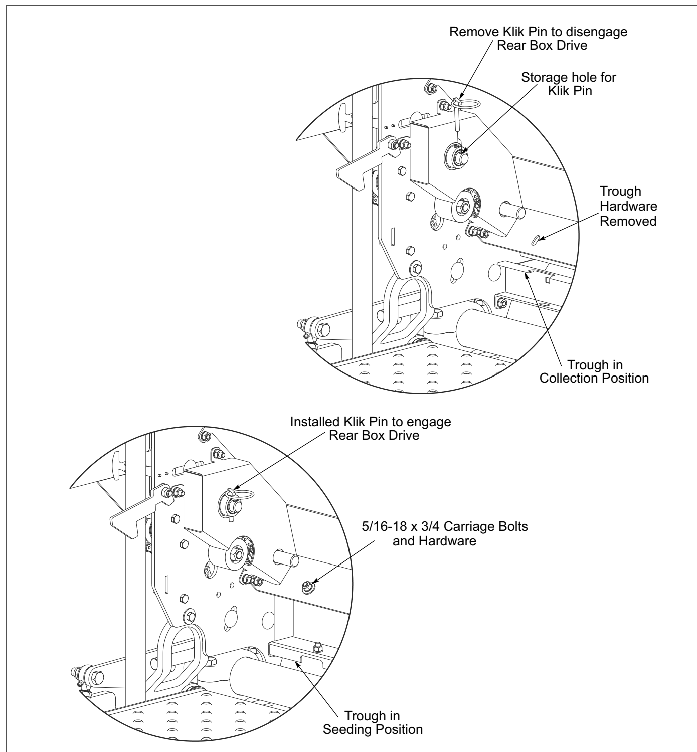
Figure 2-11: Rear Seedbox Calibration
