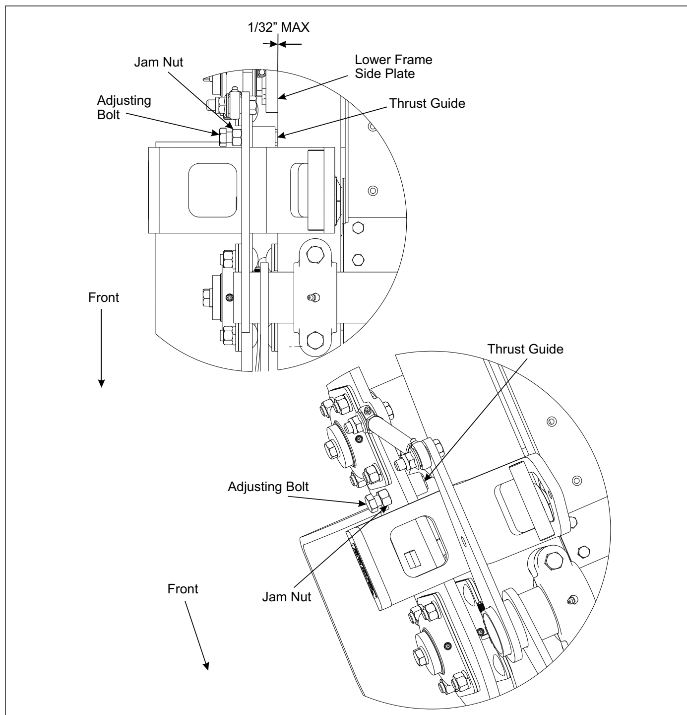
Figure 4-5: Rotor Thrust Guide
