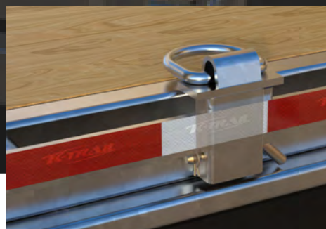
REMOVABLE D-RINGS
