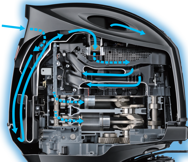
➔ Air Flow
