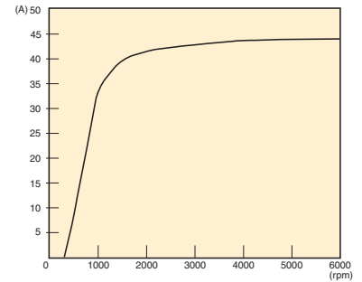
Alternator Output
