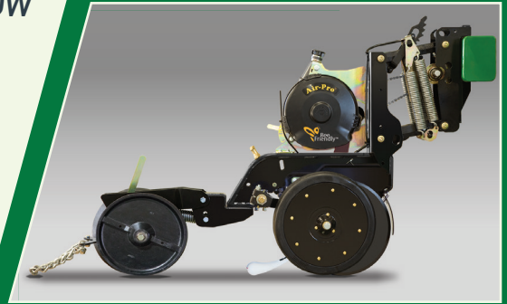
6-ROW
