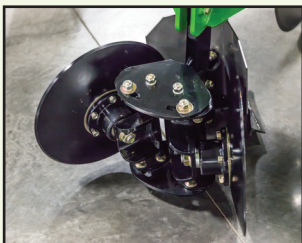
BARRING-OFF DISCS
