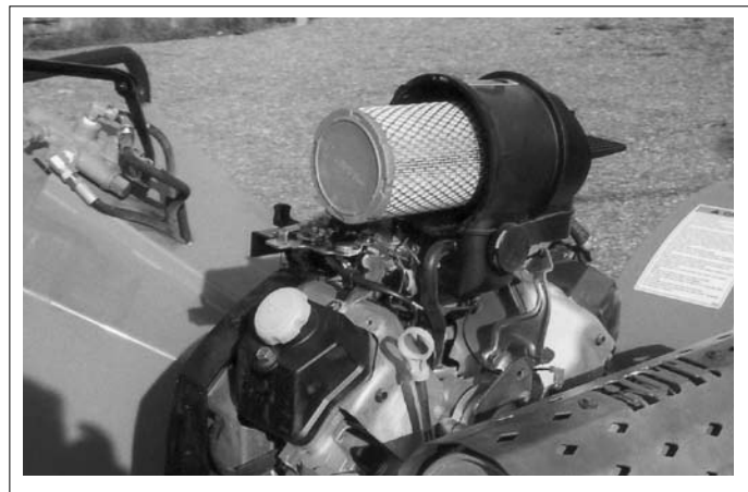
Fig. 40 AIR CLEANER
