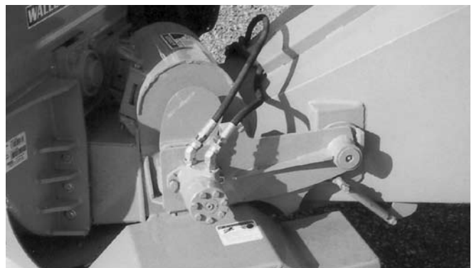
Roller Drive Motor
