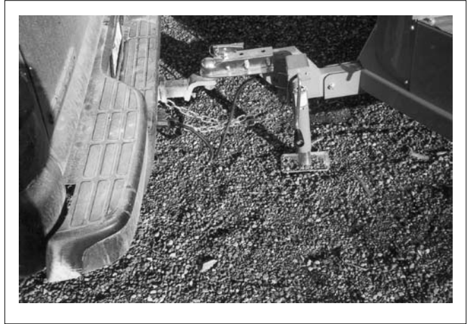
Fig. 10 STAND/WIRING HARNESS
