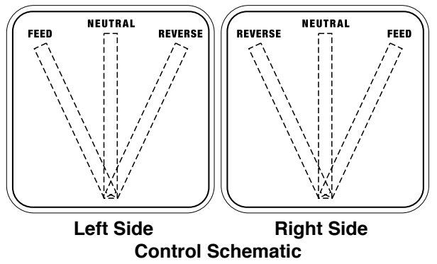
Fig. 3 HYDRAULIC FEED CONTROL LEVER
