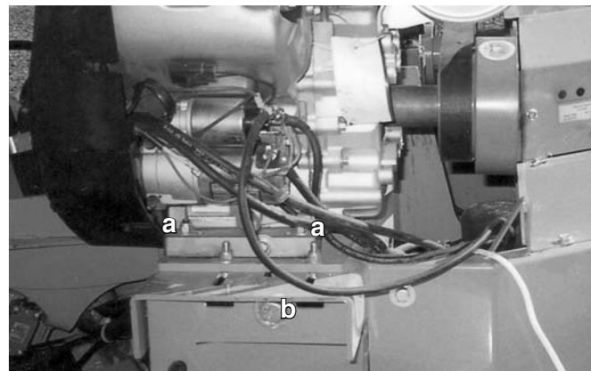
a. Engine Mounting Bolts b. Adjusting Bolt
