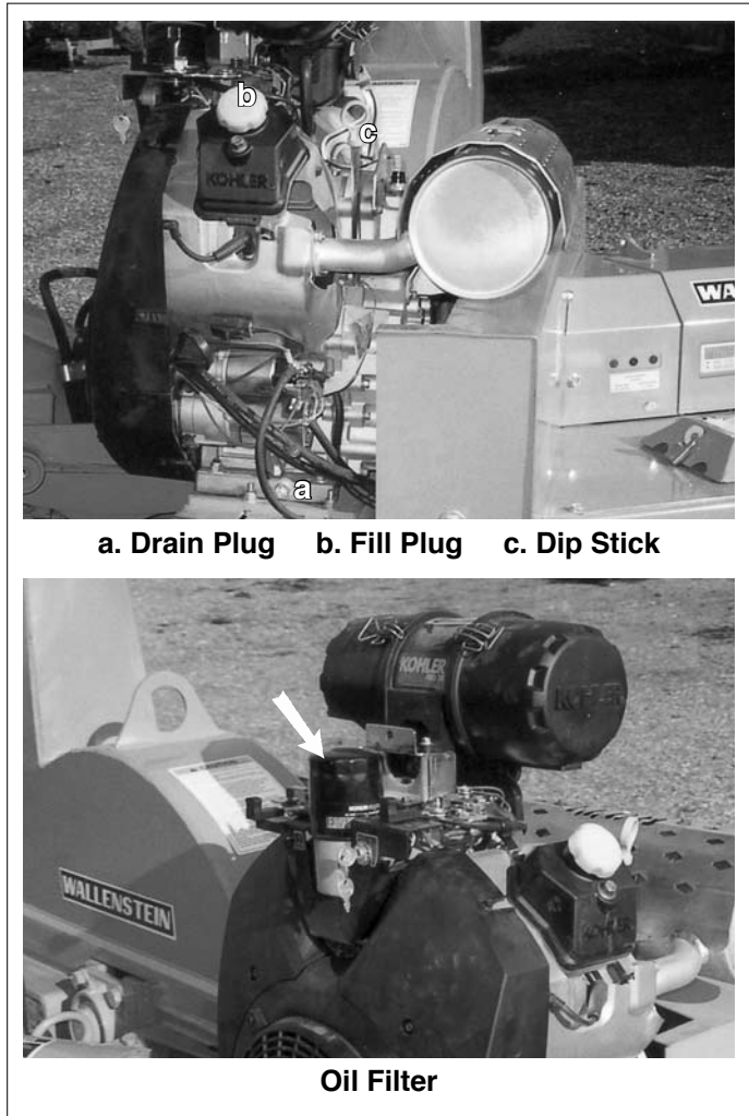
Fig. 46 ENGINE OIL
