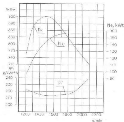
D-260.4S2 engine performance diagram
