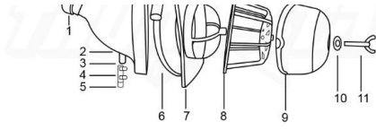
A - Assembly
