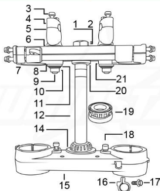
A - Assembly
