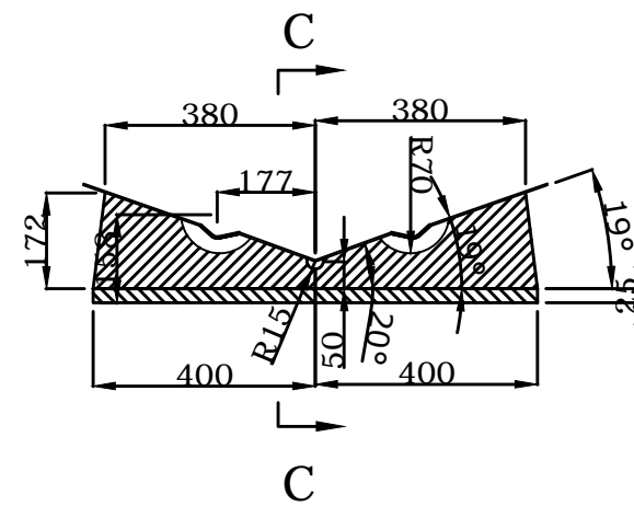
TRANSVERSAL SECTION "A"
