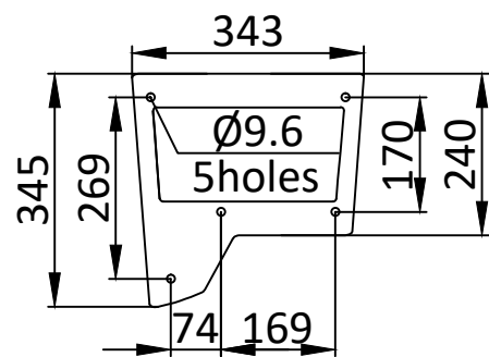
View A
