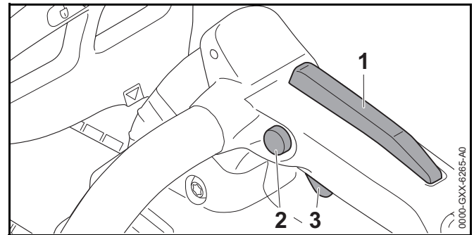
Ergo-Lever (1), Trigger Switch Lockout (2) and Trigger Switch (3)
