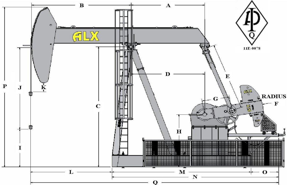
GENERAL DIMENSIONS
