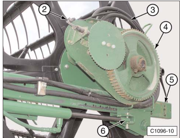
(2) Reel Speed Sensor. (3) Hydraulic Hoses. (4) Drive Gear or Pulley. (5) Stop Plate. (6) Cylinder Rod Connections.
