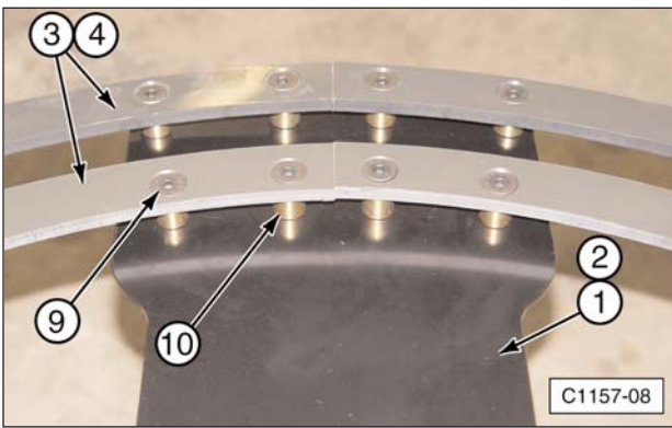
(1, 2) Track Support. (3, 4) Composite Roller Track. (9) Flathead Socket Cap Screws. (10) Spacers.
