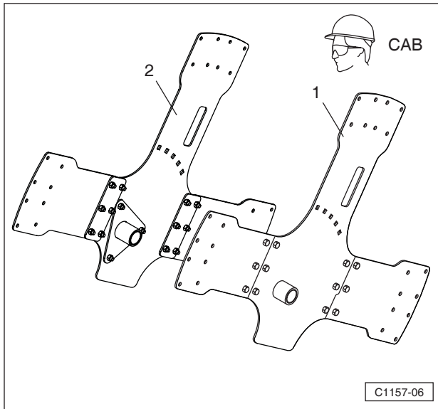
(1) Left-Hand Track Support Assembly. (2) Right-Hand Track Support Assembly.
