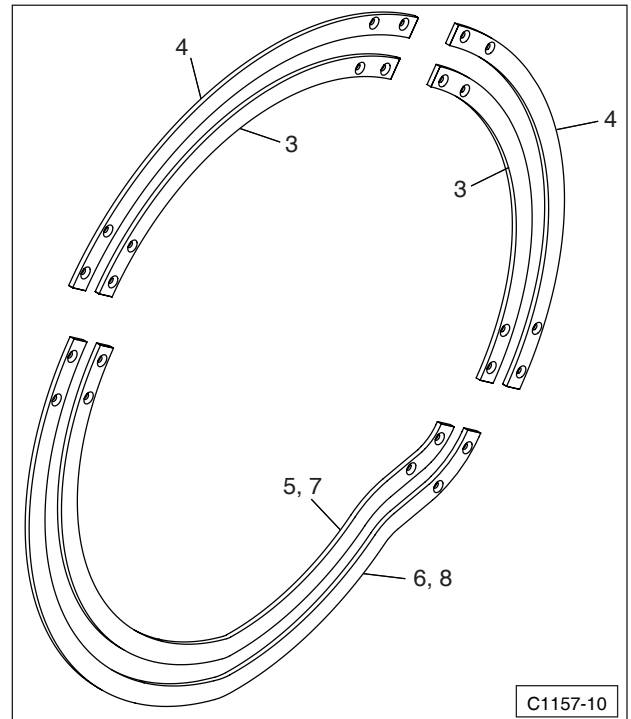
(3, 4) Composite Roller Track. (5, 7) Left-Hand and Right-Hand Inner Steel Roller Track. (6, 8) Left-Hand and Right-Hand Outer Steel Roller Track.
