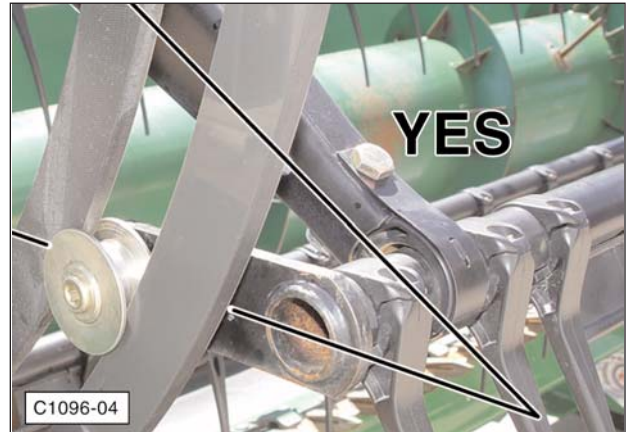
Correct orientation (roller is below or leading tine tube into header).
