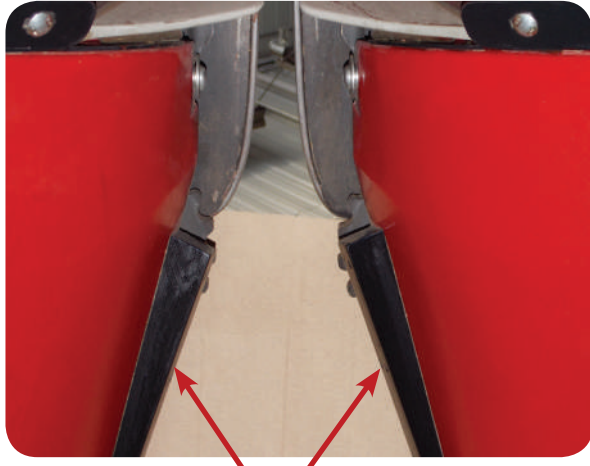
The Corn Stalk Guide maneuvers your corn past the exposed gathering chain and sprocket, into the header.
