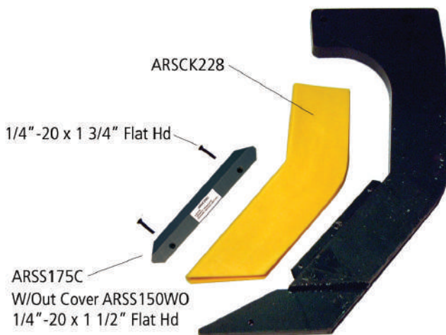
KMC Steel Shank 16-080-228 Width = 1 1/4"
