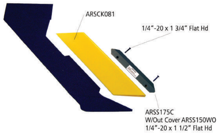
KMC Steel Shank 16-080-081 Width = 1 1/4"
