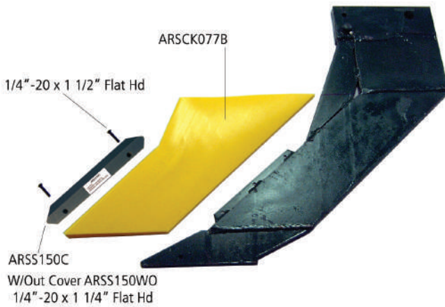
KMC Steel Shank 16-080-077 Width = 1" KMC did not change part# when brace was added.
