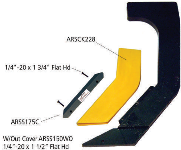
KMC Steel Shank 16-080-246 Width = 1 1/4"
