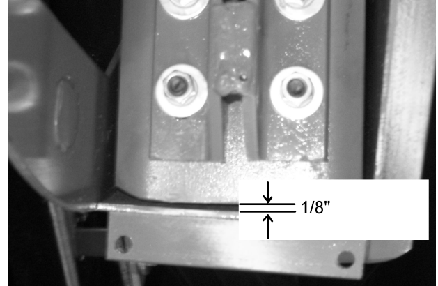
Figure 9 Blower Paddle Adjustment
