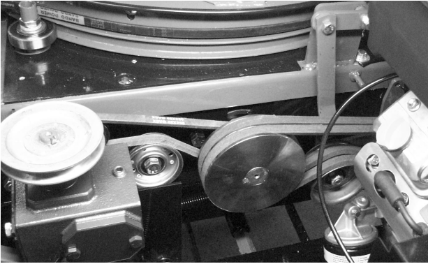
Figure 7 Rotor and Gear Box Drive Belt Installation
