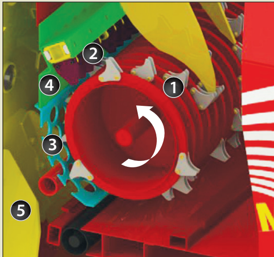
'Dual Chop' mechanism in short chop position
