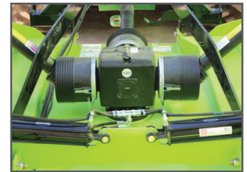
210hp (157kw) Splitter Box
