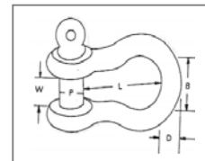
ANCHOR Screw Pin Shackle
